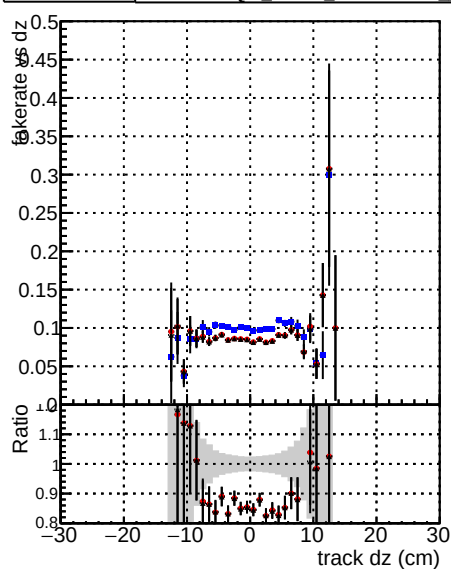
Fake rate vs d DOM V0001 R0000000001 Global cmsssw1000time RECO DOM V0001 R0000000001 Global mkFitNewO D1000time RECO DOM V0001 R0000000001 Global mkFitNewO D1000time RECO DOM V0001 R0000000001 Global mkFitNewALL 1000time RECO
