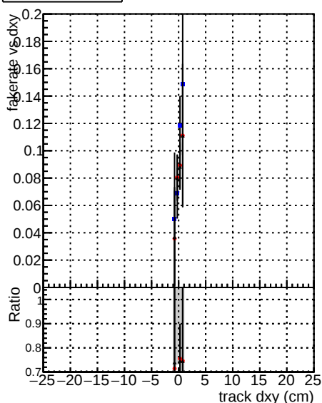
Fake rate vs d Legend DOM V0001 R0000000001 Global cmsssw1000time RECO Blue dot DOM V0001 R0000000001 Global cmsssw1000time RECO Red dot DOM V0001 R0000000001 Global mkFitNewO RECO Black dot DOM V0001 R0000000001 Global mkFitNewALL RECO
