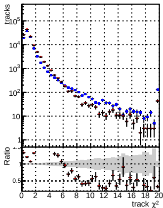
DOM V0001 R0000000001 Global cmssw1000time RECO N of reco track vs. s DOM V0001 R0000000001 Global mkFitNewOLD1000time RECO DOM V0001 R0000000001 Global mkFitNewALL1000time RECO DOM V0001 R0000000001 Global mkFitNewALL1000time RECO
