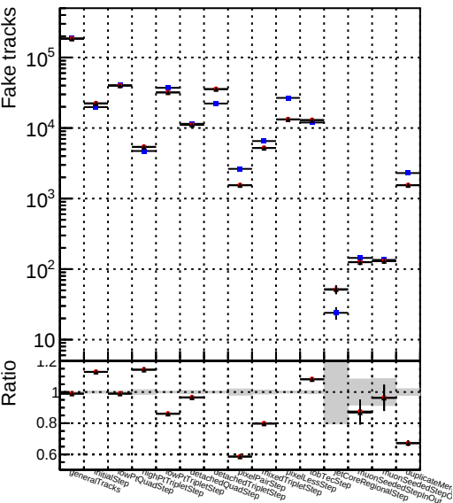
Number Legend Series Name Model Time Reco DQM_V0001_R0000000001_Global cmssw1000time RECO DQM_V0001_R0000000001_Global mkFitNewOLD1000time RECO DQM_V0001_R0000000001_Global mkFitNewALL1000time RECO
