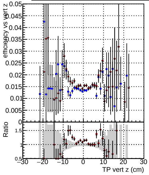
Efficiency vs vertpos —●— DQM_V0001_R000000001_Global_cmssw1000time_RECO —●— DQM_V0001_R000000001_Global_mkFitNewOLD1000time_RECO —●— DQM_V0001_R000000001_Global_mkFitNewALL1000time_RECO
