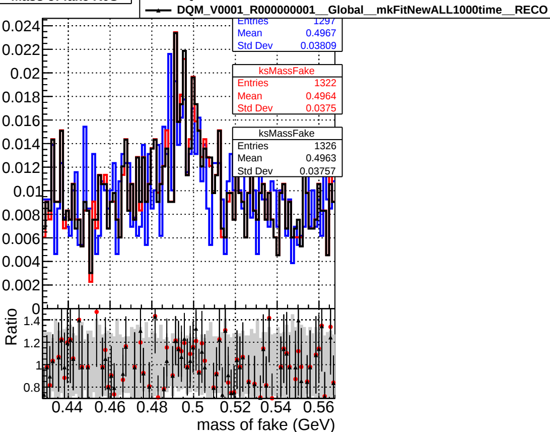
Mass of fake K0S
