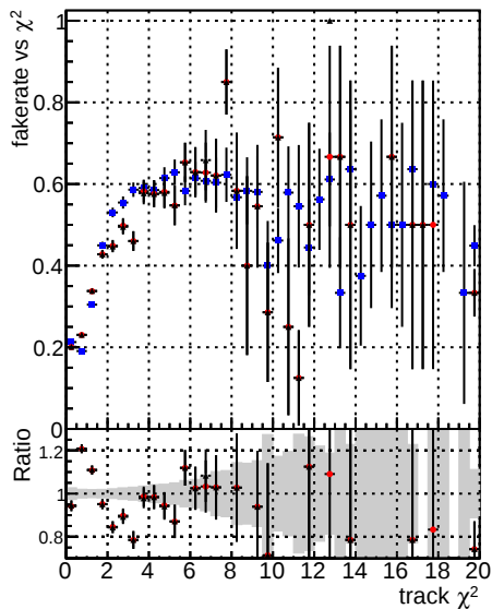
Fake rate vs. Legend DOM V0001 R0000000001 Global cmsssw1000time RECO Blue dot DOM V0001 R0000000001 Global mkEitNewO1D1000time RECO Red dot DOM V0001 R0000000001 Global mkEitNewO1D1000time RECO Black dot DOM V0001 R0000000001 Global mkEitNewO1D1000time RECO
