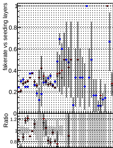
Fake rate vs. Legend DOM V0001 R0000000001 Global cmsssw1000time RECO Blue dot DOM V0001 R0000000001 Global mkEitNewO1D1000time RECO Red dot DOM V0001 R0000000001 Global mkEitNewO1D1000time RECO Black dot DOM V0001 R0000000001 Global mkEitNewO1D1000time RECO
