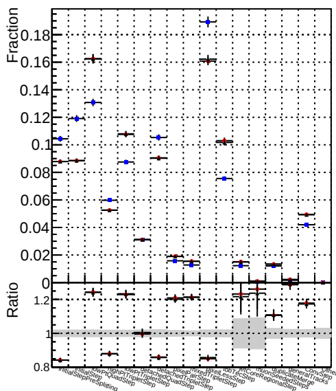
Average Legend Series DQM_V0001_R0000000001_Global_mkFitNewOLD1000time_RECO DQM_V0001_R0000000001_Global_mkFitOLD-checkDet_RECO
