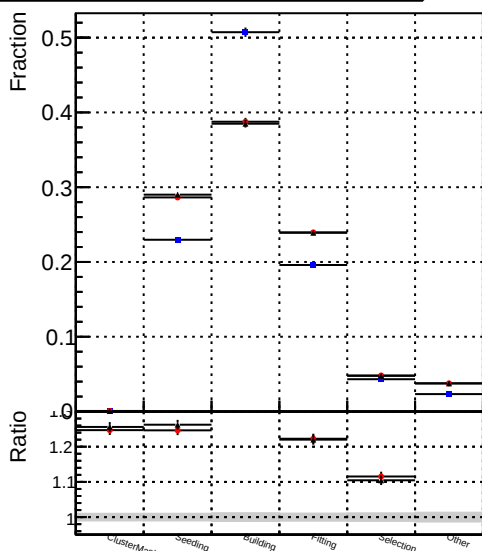
Average Legend Series DQM_V0001_R0000000001_Global_mkFitNewOLD1000time_RECO DQM_V0001_R0000000001_Global_mkFitOLD-checkDet_RECO
