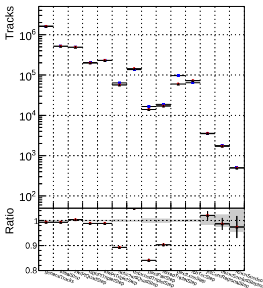
Number DQM_V0001_R000000001_Global_cmssw1000time_RECO DQM_V0001_R000000001_Global_mkFitNewOLD1000time_RECO DQM_V0001_R000000001_Global_mkFitOLD-checkDet_RECO
