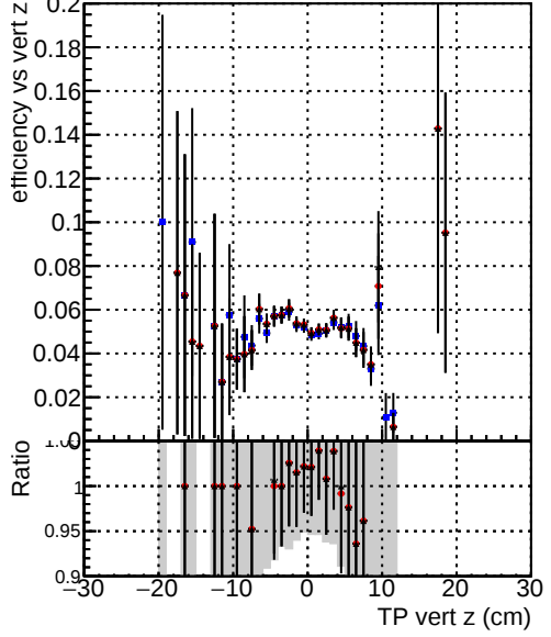
Efficiency vs vert z —●— DQM_V0001_R000000001_Global_cmssw1000time_RECO —●— DQM_V0001_R000000001_Global_mkFitNewOLD1000time_RECO —●— DQM_V0001_R000000001_Global_mkFitOLD-checkkDet_RECO
