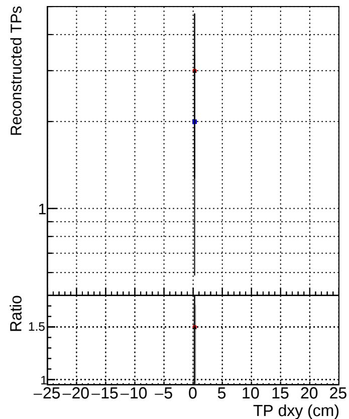
N of simulated track ■ DQM_V0001_R000000001 Global cmssw1000time RECO ● DQM_V0001_R000000001 Global mkFitNewOLD1000time RECO ▲ DQM_V0001_R000000001 Global mkFitOLD-checkDet RECO
