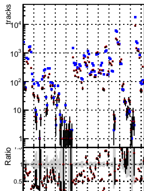
N of reco track vs. s DQM V0001 R0000000001 Global cms-sw-1000time RECO DQM V0001 R0000000001 Global mkFitNewOLD1000time RECO DQM V0001 R0000000001 Global mkFitTOLD-checkdet RECO
