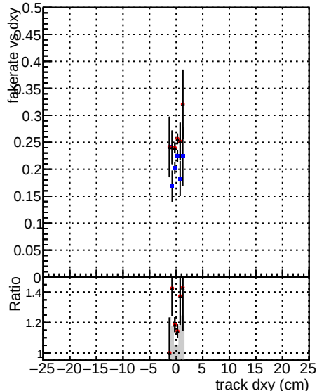
DOM_V0001 R0000000001 Global_cmssw1000time_RECO DOM_V0001 R0000000001 Global_mkeutOLD1000time_RECO DOM_V0001 R0000000001 Global_mkeutOLD-checkDet_RECO
