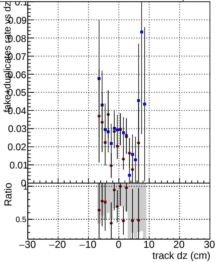
DQM_V0001_R000000001_Global_cmssw1000time_RECO DQM_V0001_R000000001_Global_mkFitNewOLD1000time_RECO DQM_V0001_R000000001_Global_mkFitOLD-checkDet_RECO
