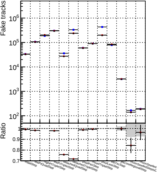
Number ● DQM_V0001_R000000001_Global_mkFitNewOLD1000time_RECO ▲ DQM_V0001_R000000001_Global_mkFitOLD-checkDet_RECO
