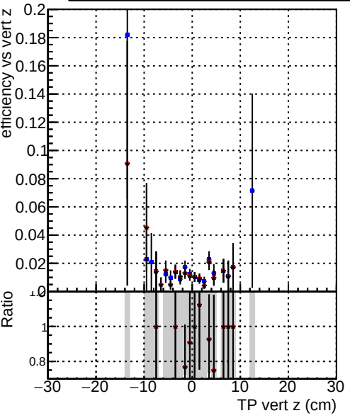
Efficiency vs vertpos —●— DQM_V0001_R0000000001_Global_cmssw1000time_RECO —●— DQM_V0001_R0000000001_Global_mkFitNewOLD1000time_RECO —●— DQM_V0001_R0000000001_Global_mkFitOLD-checkDet_RECO
