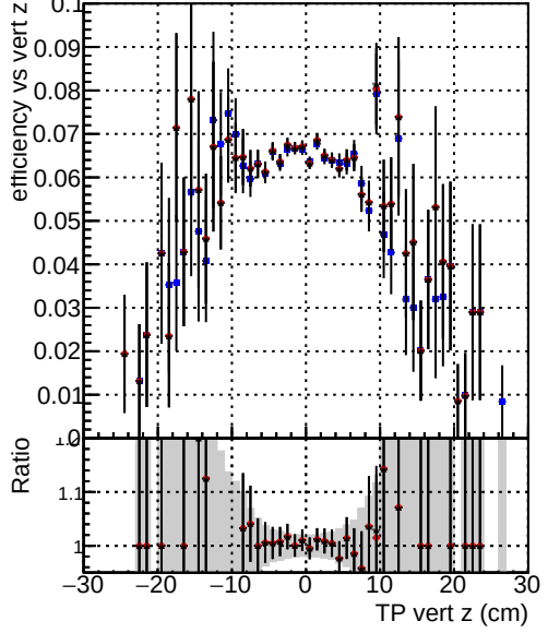
Efficiency vs. TP vert z (cm) —●— DQM_V0001_R0000000001_Global_cmssw1000time_RECO —●— DQM_V0001_R0000000001_Global_mkFitNewOLD1000time_RECO —●— DQM_V0001_R0000000001_Global_mkFitOLD-checkDet_RECO
