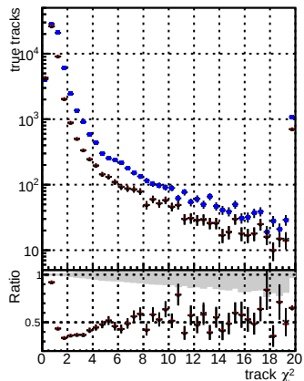
N of reco track vs. DQM_V0001 R00000000001 Global mkFitNewOLD100time RECO DQM_V0001 R00000000001 Global mkFitOld-checkDet RECO
