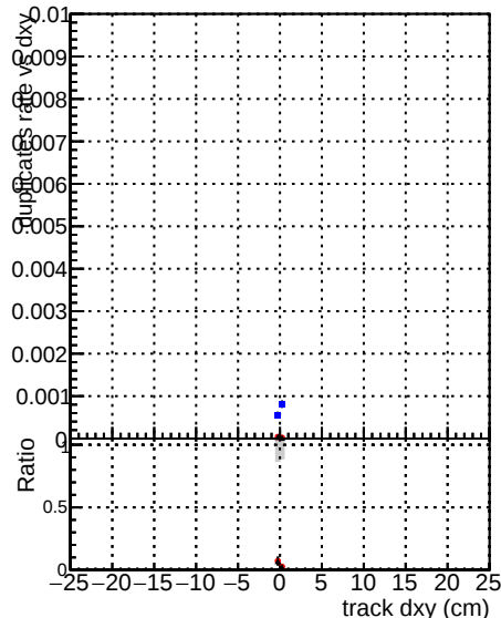
Global cmssw1000time RECO Global mkViewOLD1000time RECO Global mkFOLD-checkDet RECO
