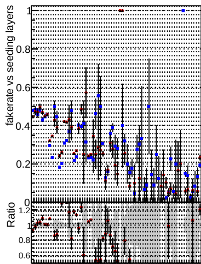
Fake rate vs. DOM V0001 R0000000001 Global cms-sw1000time RECO DOM V0001 R0000000001 Global mktFOLD1000time RECO DOM V0001 R0000000001 Global mktFOLD-checkDet RECO
