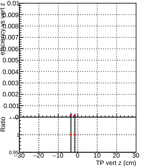
Efficiency vs. TP vert z (cm) Legend: DQM_V0001_R0000000001_Global_mkFitNewOLD1000time_RECO DQM_V0001_R0000000001_Global_mkFitOLD-checkDet_RECO
