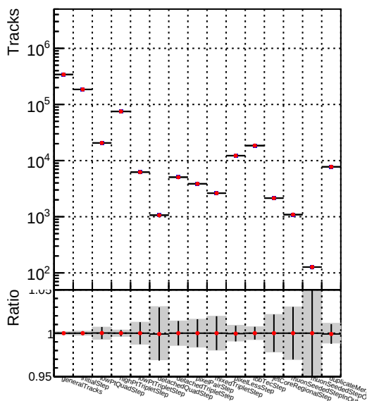
DQM_V0001_R000000001_Global_mkFitNewOLD1000time_RECO
