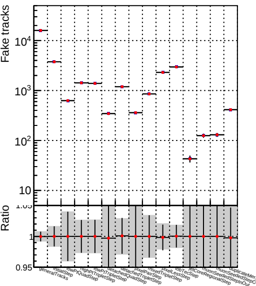
Numbe —●— DQM_V0001_R000000001_Global_mkFitOLD-checkDet_RECO
