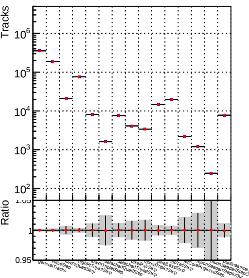
DQM_V0001_R000000001__Global__mkFitNewOLD1000time__RECO
