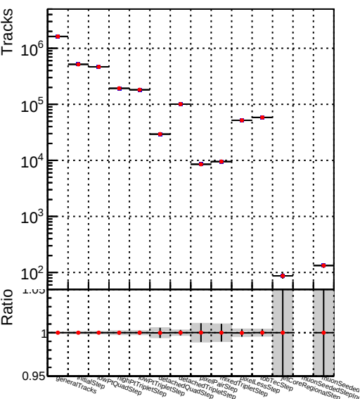
DQM_V0001_R0000000001_Global_mkFitNewOLD1000time_RECO
