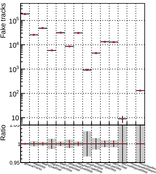
Number —●— DQM_V0001_R000000001_Global_mkFitOLD-checkDet_RECO
