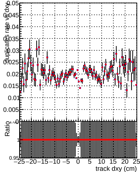
Global mkFitNewOLD1000time RECO DQM_V0001_R0000000001 Global mkFitOLD-checkDet RECO DQM_V0001_R0000000001
