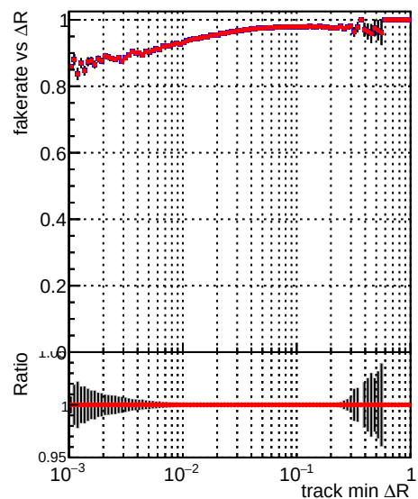
—●— DQM_V0001_R000000001_Global_mkFitNewOLD1000time_RECO —●— DQM_V0001_R000000001_Global_mkFitOLD-checkDet_RECO
