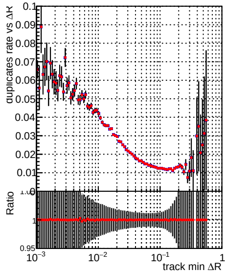
—●— DQM_V0001_R000000001_Global_mkFitNewOLD1000time_RECO —●— DQM_V0001_R000000001_Global_mkFitOLD-checkDet_RECO
