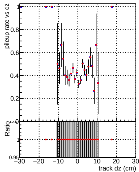
Global mkFitOLD-checkDet RECO
