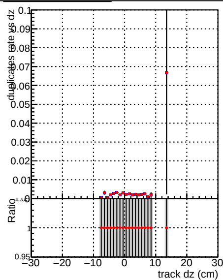
—•— DQM_V0001_R0000000001_Global_mkFitNewOLD1000time_RECO —•— DQM_V0001_R0000000001_Global_mkFitOLD-checkDet_RECO
