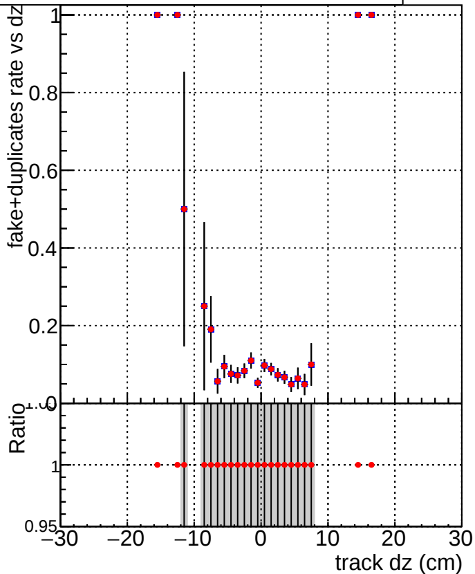
DQM_V0001_R0000000001_Global_mkFitNewOLD1000time_RECO
