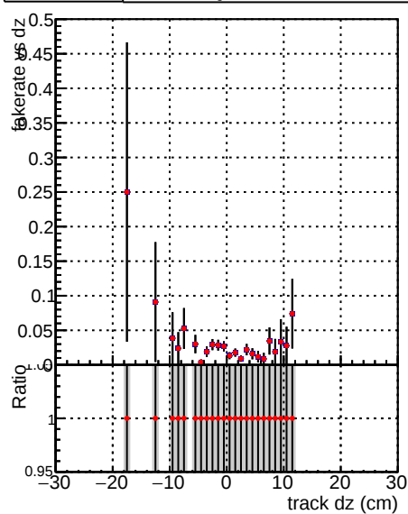
—•— DQM_V0001_R0000000001_Global_mkFitNewOLD1000time_RECO —•— DQM_V0001_R0000000001_Global_mkFitOLD-checkDet_RECO
