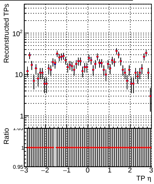
— DQM_V0001_R0000000001_Global_mkFitNewOLD1000time_RECO — DQM_V0001_R0000000001_Global_mkFitOLD-checkDet_RECO
