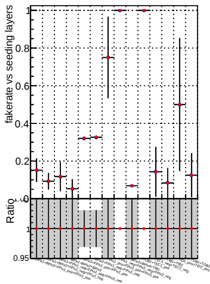
Fake rate vs. DQM_V0001_R000000001 Global mkFitNewOLD1000time RECO DQM_V0001_R000000001 Global mkFitOLD-checkDet RECO
