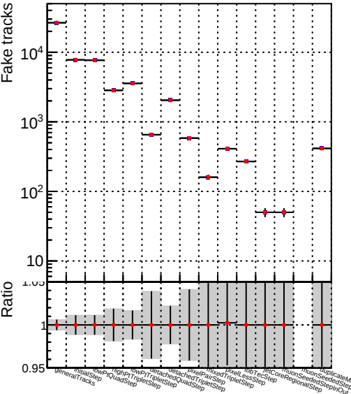
Number ● DQM_V0001_R000000001_Global_mkFitOLD-checkDet_RECO
