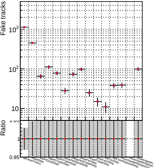
Numbe —●— DQM_V0001_R000000001_Global_mkFitOLD-checkDet_RECO
