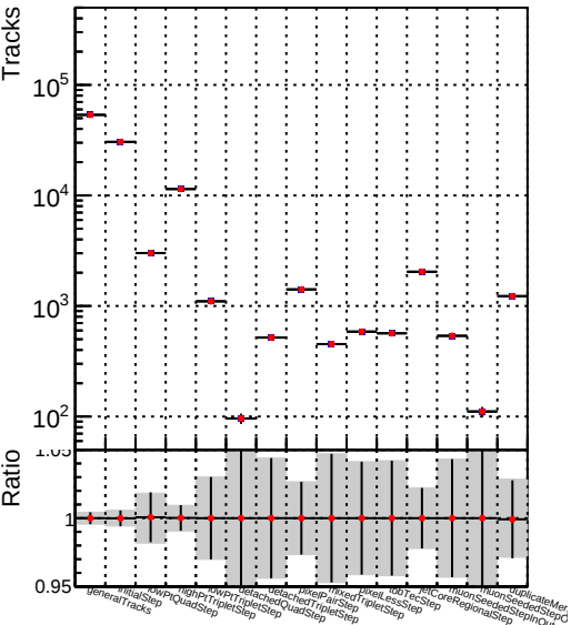
DQM_V0001_R000000001__Global__mkFitNewOLD1000time__RECO
