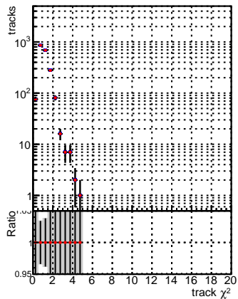
N of reco track vs. \chi^2 for different fit models
