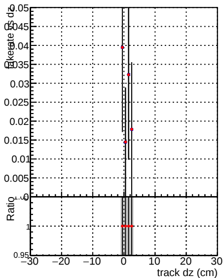
█ DQM_V0001_R0000000001 Global mkFitNewOLD1000time RECO █ DQM_V0001_R0000000001 Global mkFitOLD-checkDet RECO
