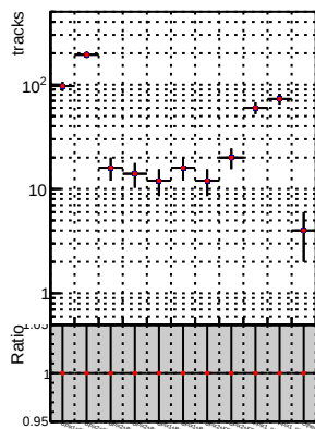
N of reco track vs. \chi^2 — Global_mkFitNewOLD1000time_RECO — Global_mkFitOLD-checkDet_RECO
