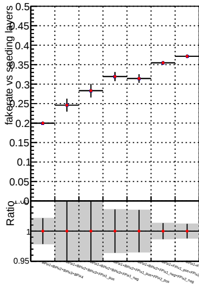
Fake rate vs. █ ● DQM_V0001_R000000001 Global mkFitNewOLD1000time RECO █ ● DQM_V0001_R000000001 Global mkFitOLD-checkDet RECO
