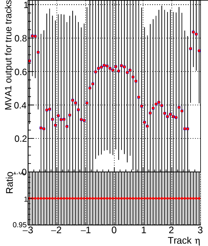
MVA1 of associated tracks (recoToSim) vs. track \eta ■ DQM_V0001_R000000001_Global_mkFitNewOLD1000time_RECO ● DQM_V0001_R000000001_Global_mkFitOLD-checkDet_RECO
