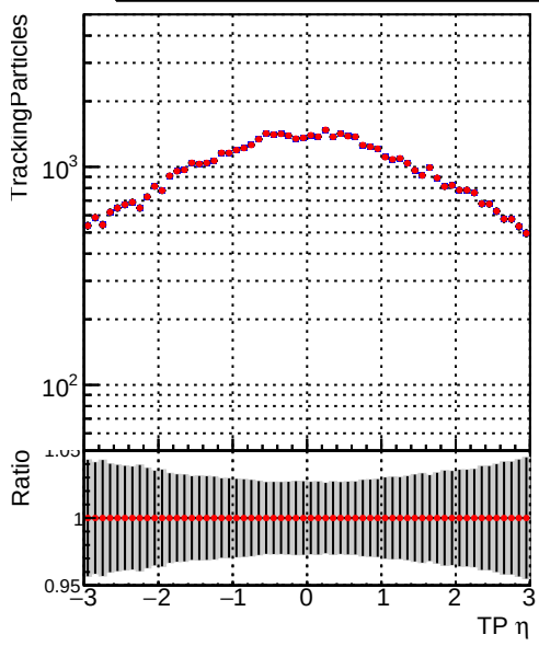
—●— DQM_V0001_R000000001_Global_mkFitNewOLD1000time_RECO —●— DQM_V0001_R000000001_Global_mkFitOLD-checkDet_RECO
