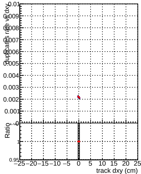
—●— DQM_V0001_R0000000001_Global_mkFitNewOLD1000time_RECO —●— DQM_V0001_R0000000001_Global_mkFitOLD-checkDet_RECO
