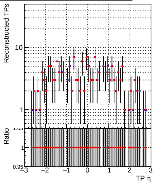
— DQM_V0001_R000000001_Global_mkFitNewOLD1000time_RECO — DQM_V0001_R000000001_Global_mkFitOLD-checkDet_RECO
