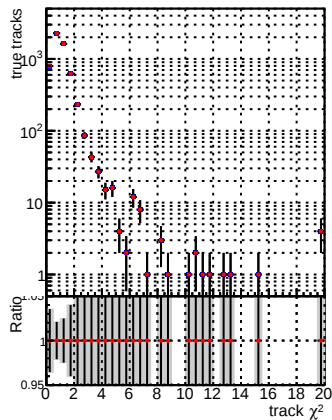
N of reco track vs. \chi^2 — Global_mkFitNewOLD1000time_RECO — Global_mkFitOLD-checkDet_RECO
