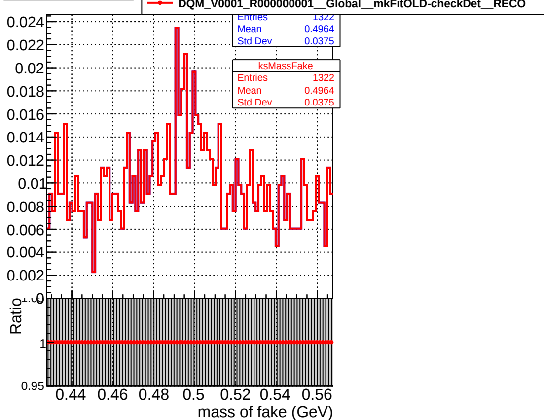
Mass of fake K0S
