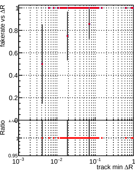
DQM_V0001_R000000001_Global_mkFitNewOLD1000time_RECO DQM_V0001_R000000001_Global_mkFitOLD-checkDet_RECO
