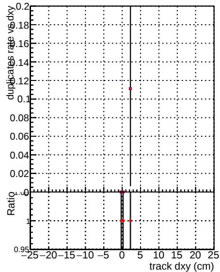
—●— DQM_V0001_R0000000001_Global_mkFitNewOLD1000time_RECO —●— DQM_V0001_R0000000001_Global_mkFitOLD-checkDet_RECO
