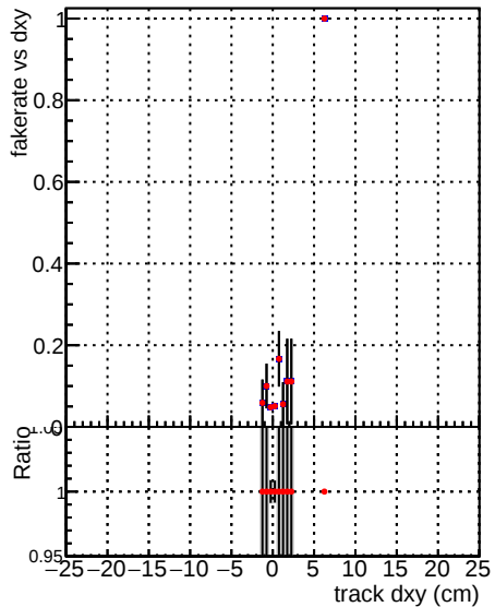
—●— DQM_V0001_R0000000001_Global_mkFitNewOLD1000time_RECO —●— DQM_V0001_R0000000001_Global_mkFitOLD-checkDet_RECO
