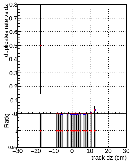
—●— DQM_V0001_R0000000001_Global_mkFitNewOLD1000time_RECO —●— DQM_V0001_R0000000001_Global_mkFitOLD-checkDet_RECO
