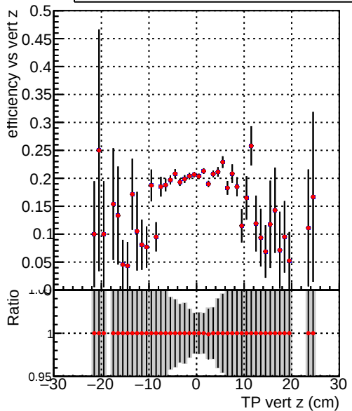
Efficiency vs vert z — DQM_V0001_R000000001_Global_mkFitNewOLD1000time_RECO — DQM_V0001_R000000001_Global_mkFitOLD-checkDet_RECO
