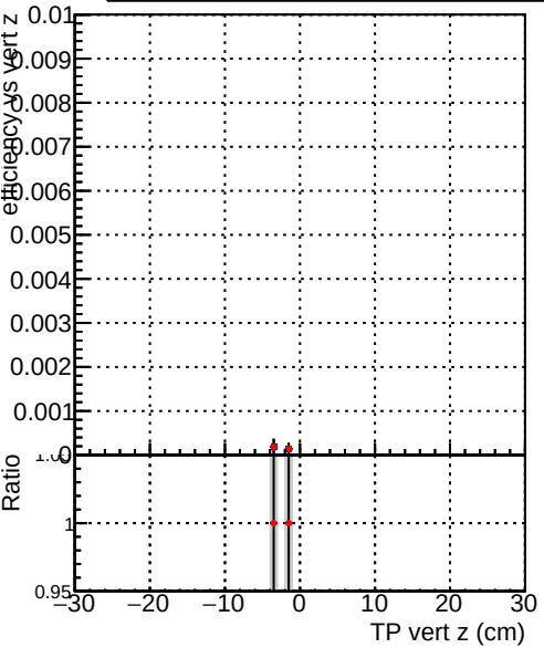
Efficiency vs. TP vert z Legend: DQM_V0001_R0000000001_Global_mkFitNewOLD1000time_RECO DQM_V0001_R0000000001_Global_mkFitOLD-checkDet12_RECO
