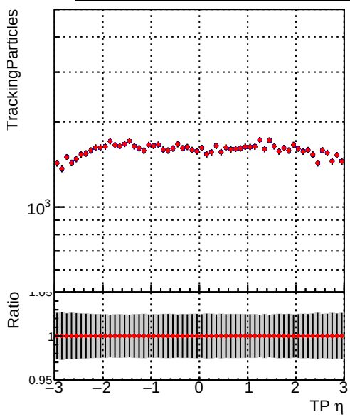
Legend: DQM_V0001_R0000000001_Global_mkFitNewOLD1000time_RECO (blue line), DQM_V0001_R0000000001_Global_mkFitOLD-checkDet12_RECO (red line)
