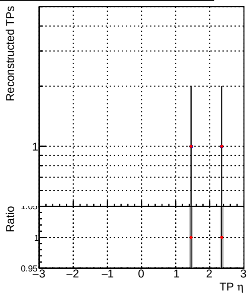
Legend: DQM_V0001_R0000000001_Global_mkFitNewOLD1000time_RECO (blue line), DQM_V0001_R0000000001_Global_mkFitOLD-checkDet12_RECO (red line)
