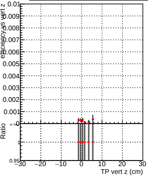
Efficiency vs. TP vert z (cm) Legend: DQM_V0001_R0000000001_Global_mkFitNewOLD1000time_RECO DQM_V0001_R0000000001_Global_mkFitOLD-checkDet12_RECO
